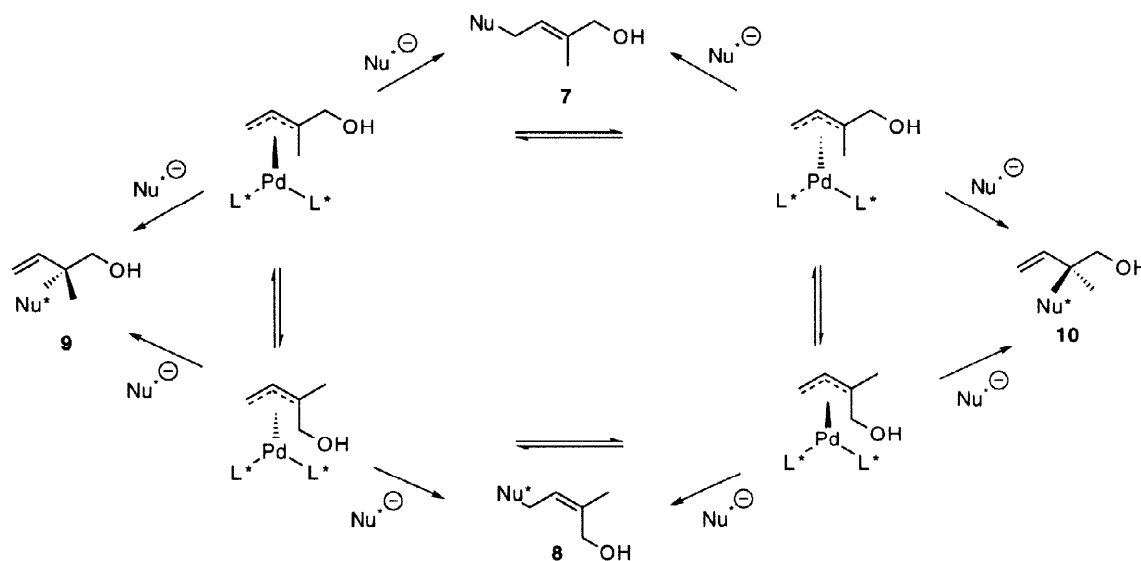
Scheme 1. Selectivity Issues in Reactions of Isoprene Monoepoxide
